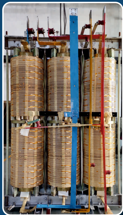
NEW COIL ASSEMBLY
