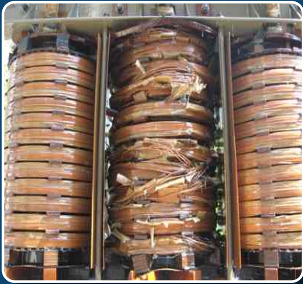
1500 KVA BEFORE REWINDING
