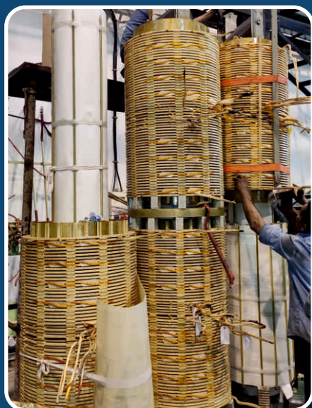
AFTER CORE & COIL ASSEMBLY
