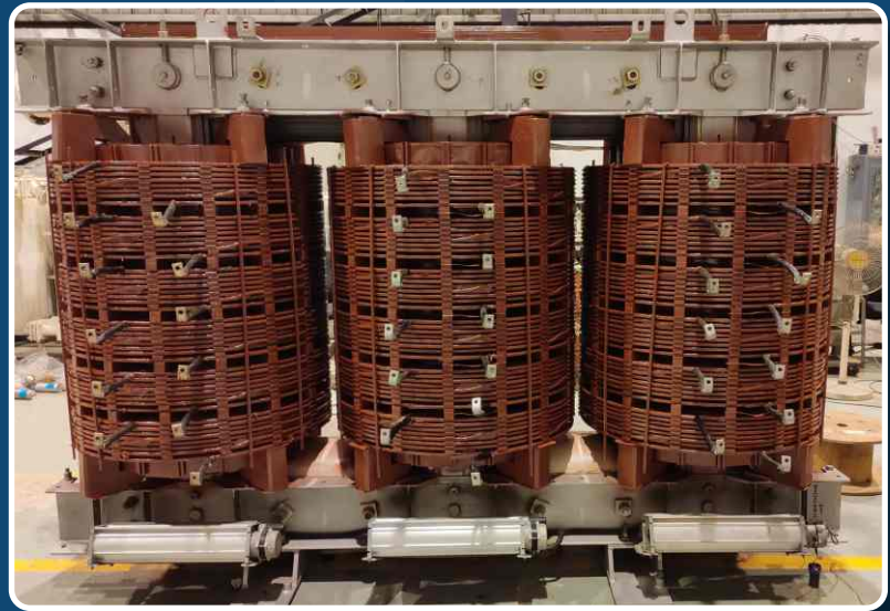
11 MVA FAULTY TRANSFORMER
