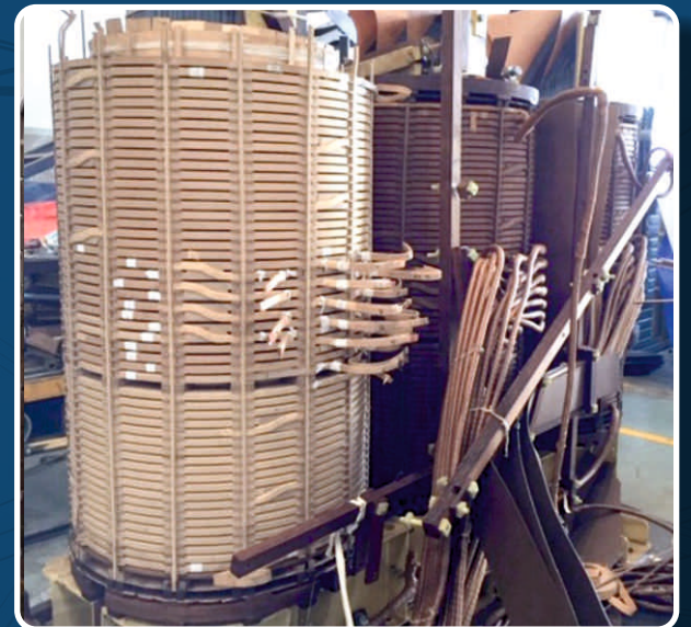
NEW COIL REWIND
