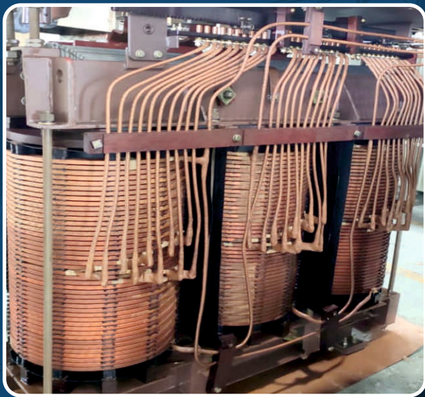
2 MVA BEFORE REWINDING
