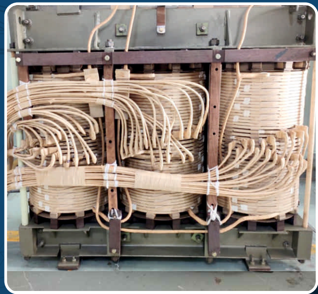
2 MVA AFTER REWINDING
